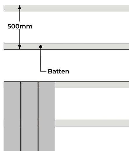
Vertical Installation
